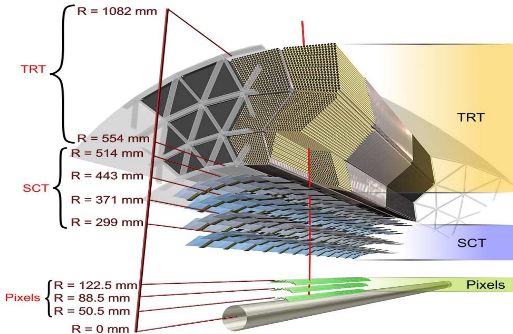
Figure 3: The above graphic shows the positions, sizes, and placements of each of the three technologies in the inner detector in relation to each other. ATLAS Experiment © 2014 CERN
