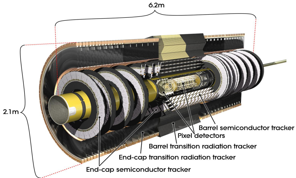
Figure 1: Above is a computer rendered cross sectional model of the ATLAS inner detector. ATLAS Experiment © 2014 CERN
