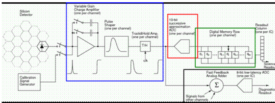
Figure 2.57: Block diagram of BeamCal Front-End Integrated Circuit.
