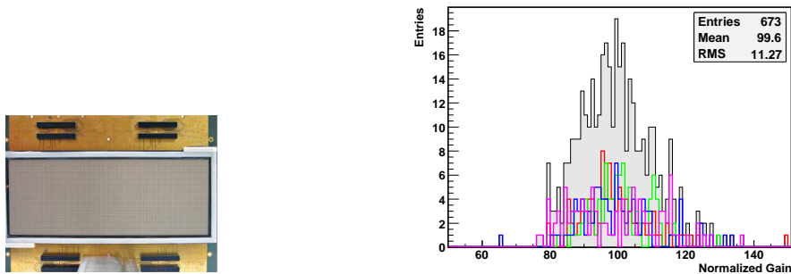
Figure 2.29: MICROMEAS 12×32 cm 2 analog readout prototype with 1 cm 2 pads. MPV dispersion normalized to 100 % for four prototypes
