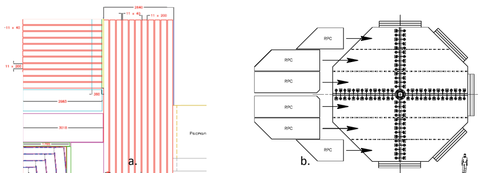
Figure 2.41: (a) Quarter-section of the SiD flux return. (b) Sub-division of the endcap into RPC modules.
