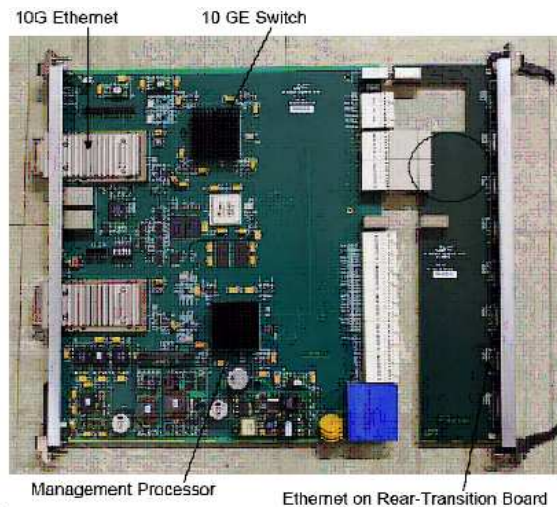
Figure 2.55: SLAC ATCA Cluster Interconnect Module.
