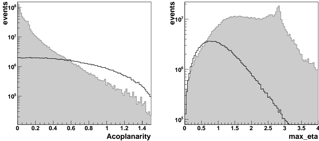
Figure 4.25: Examples of selection variables: acoplanarity (left) and maximum pseudorapidity (right) of jets. Signal with m_{\tilde{b}} = 230 GeV and m_{\tilde{\chi}_1^0} = 210 GeV (black) is shown together with the inclusive SM background (filled histogram). The signal was scaled up by a factor of 100000.
