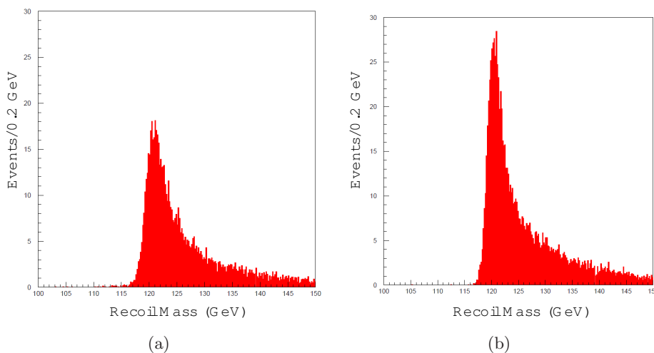
Figure 4.2: Recoil mass distributions following selection cuts for eeH (a) and \mu\mu H (b) assuming 250 \text{ fb}^{-1} luminosity with 80eR initial state polarization. Background is not included.
