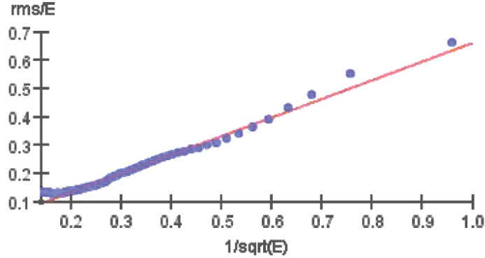
Figure 2.33: Resolution plot for single neutral hadrons from t\bar{t} events. The line in the resolution plot represents 65\%/E_{Gen} .
