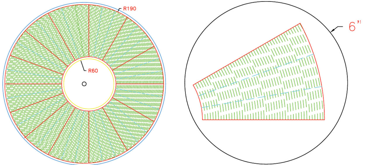
Figure 2.44: LumiCal sensor and segmentation.
