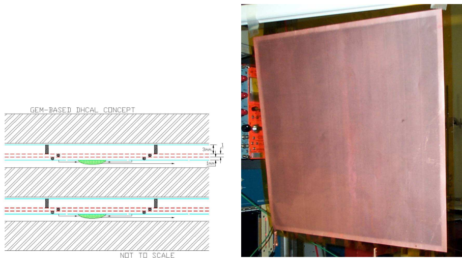
Figure 2.28: Left: GEM DHCAL Concept. Right: A 30 cm x 30 cm foil from 3M Corporation.
