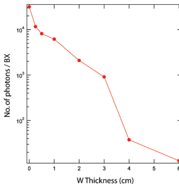
Figure 2.50: Number of photons penetrating the tungsten mask as a function of the mask thickness
