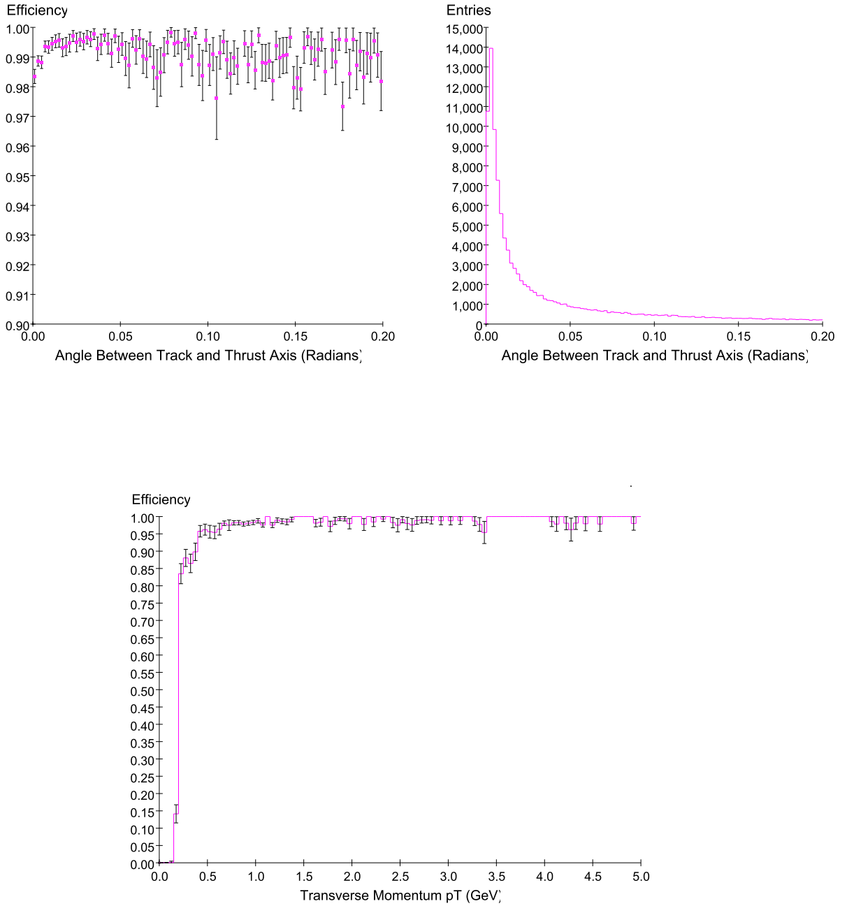
Figure 2.12: Tracking efficiency as function of \alpha (upper left) and distribution in \alpha (upper right) for e^+e^- \rightarrow q\bar{q} events at \sqrt{s} = 1 TeV. The bottom figure shows the tracking efficiency for e^+e^- \rightarrow b\bar{b} events at \sqrt{s} = 500 GeV with the background from 10 bunch crossings overlaid.
