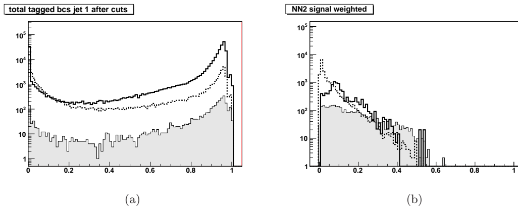
Figure 4.8: Four jet channel: (a) Flavour tag 'c with b only background' for the first jet; (b) NN_{Higgs-signal} output. Solid curves are SM background, dashed curves are inclusive Higgs sample and filled histograms are the signal.
