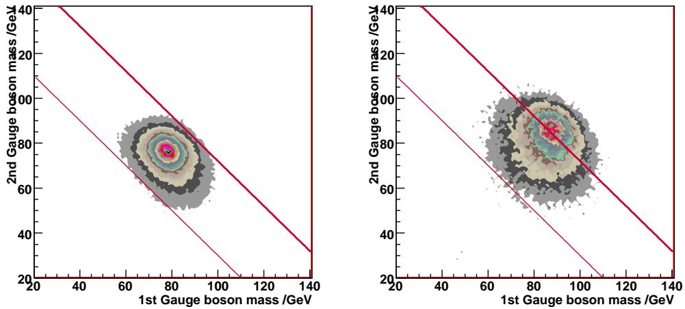
Figure 4.21: The reconstructed boson masses from the four jets, selecting chargedino events. Left: pure chargedino signal; right: pure neutralino signal. The region between the two straight lines shows the allowed chargedino selection window.
