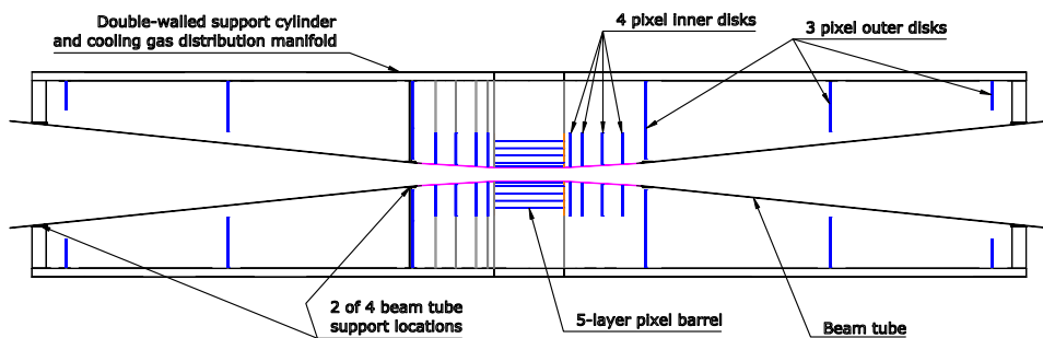
Figure 2.1: R-z view of the vertex detector. The right hand side has been drawn without the support structures.
