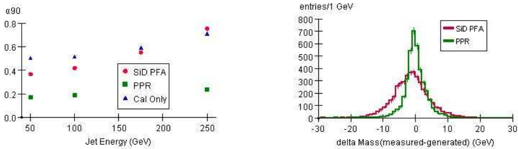
Figure 2.34: Left: \alpha_{90} vs jet energy for the 3 different reconstructions. Right: Mass residuals in the ZZ test sample. For PPR \text{rms}_{90} = 2.2 GeV. For SiD PFA \text{rms}_{90} = 4.0 GeV
