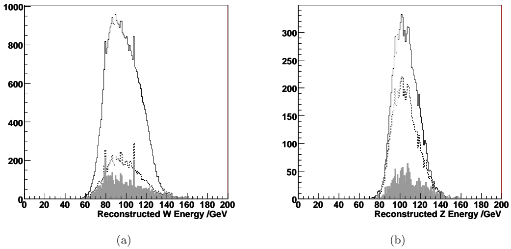
Figure 4.22: (a) The stack histogram of reconstructed W energy for the chargedino selection. The solid line shows the combined chargedino signal and all backgrounds including neutralino, the dashed line is neutralino events and SM background, the solid grey line is the SM background only. (b) Reconstructed Z energy for neutralino selection, the solid line is the neutralino signal and all backgrounds including chargedino, dashed line is the chargedino events and SM background, the solid grey line is the SM background only. The spikes in (a) are due to the large weight of a few events in the SM background sample.
