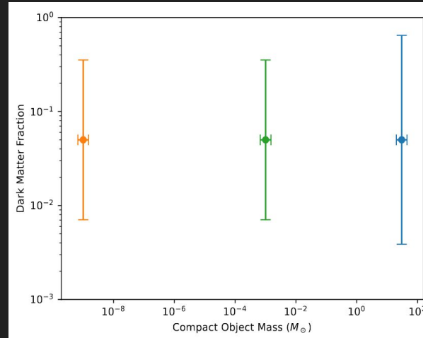
Primordial black holes w/ Rubin/Roman
