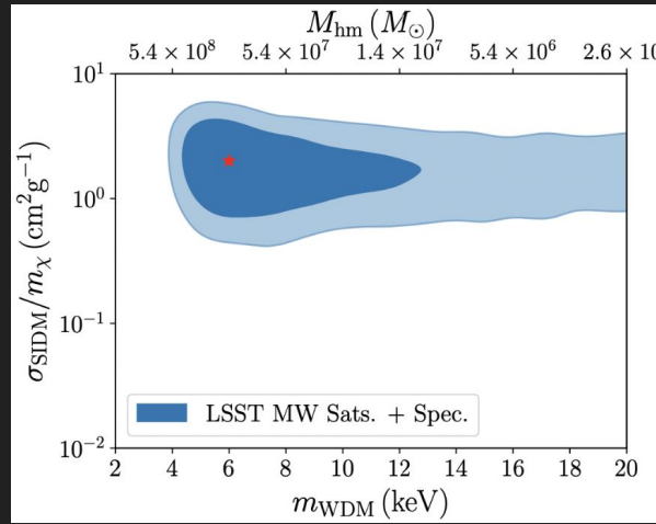
SDIM/WDM w/ Rubin LSST (the plot needs updated)
