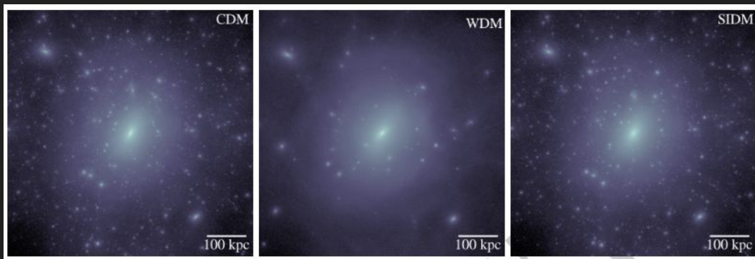
Replaced simulation analysis complexity figure with pretty pictures of simulations (Bullock & Boylan-Kolchin 2017)
