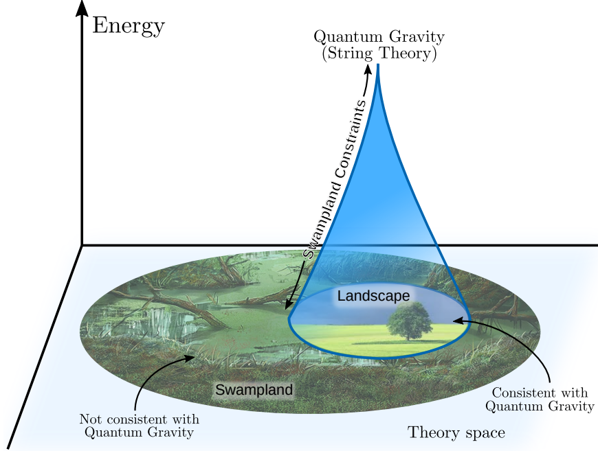
Figure 7: The swampland and landscape of EFTs. The space of consistent EFTs forms a cone because swampland constraints become stronger at high energies. From Ref. [634].
