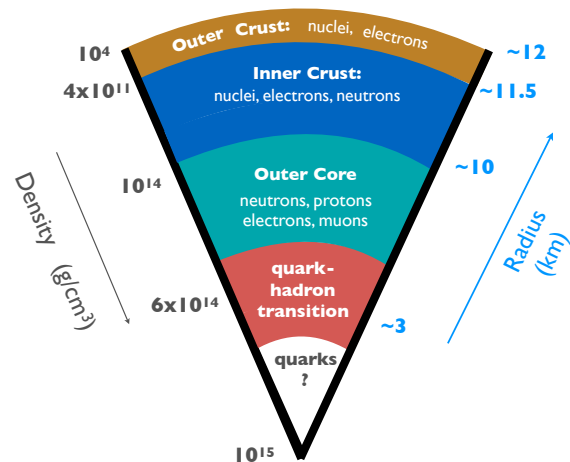
Figure 4: The structure of a neutron star as predicted by theory.
